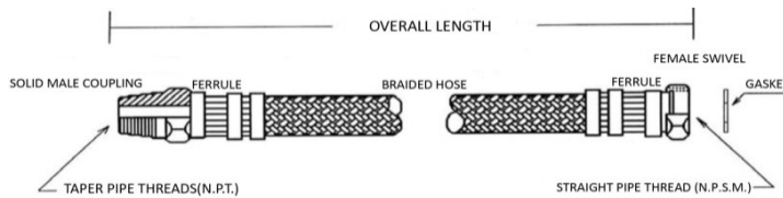
Male Coupling (Shown Above)
